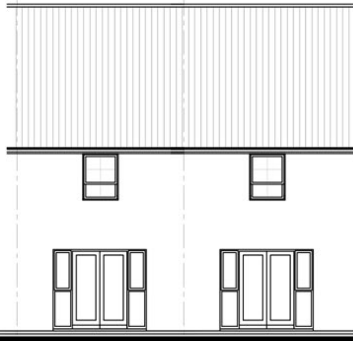
REAR ELEVATION
